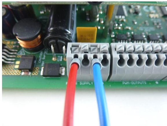
Figure 35: Power connection to the PiXtend V2 -S-
