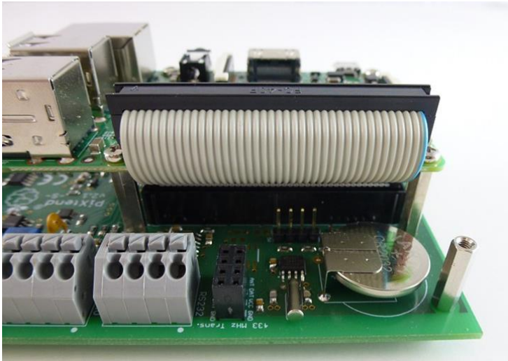
Figure 41: Connection between the PiXtend V2 -S- and Raspberry Pi
