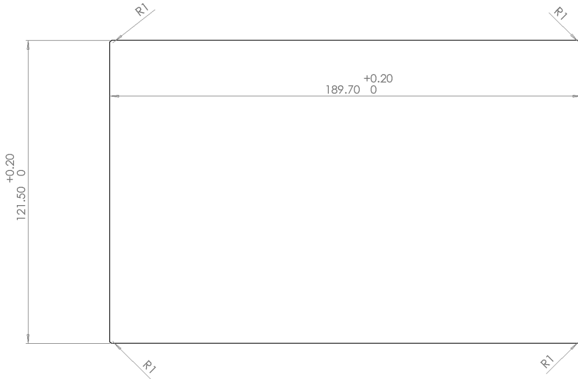
Figure 5: Mounting cut-out
