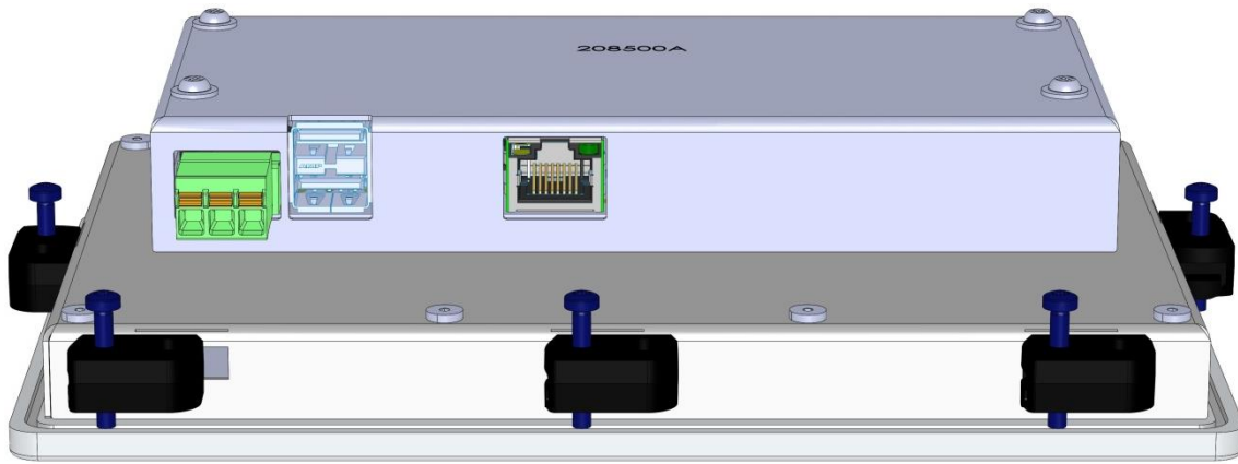
Figure 8: Side view from below
